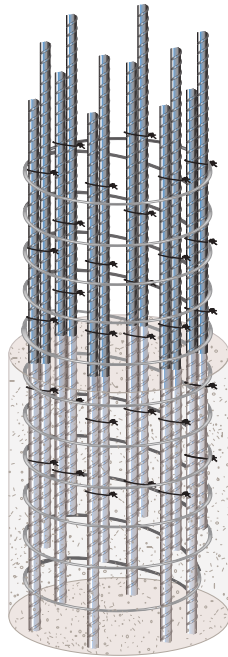
Lap splicing inhibits concrete consolidation
