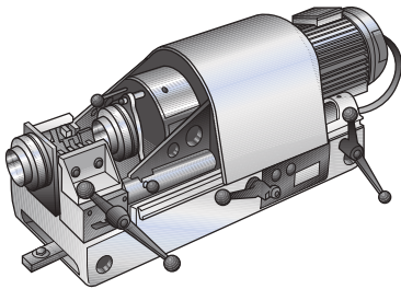
nVent LENTON bar threading machine EL-BT-101 Net weight 178 kg (392 lbs). Cutting oil capacity 14 liters (3.7 gal).
