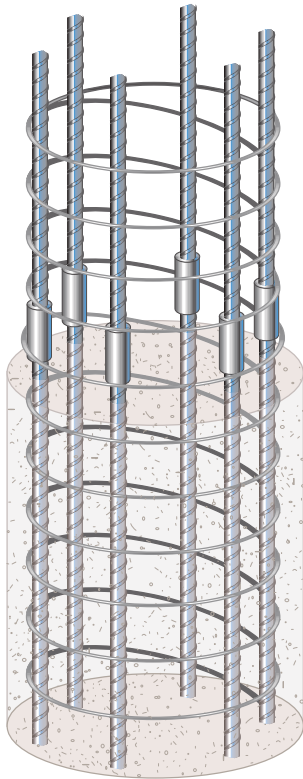
nVent LENTON mechanical splices
